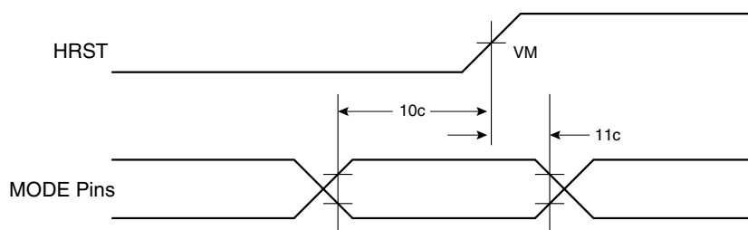
Figure 9. Mode Select Input Timing Diagram
