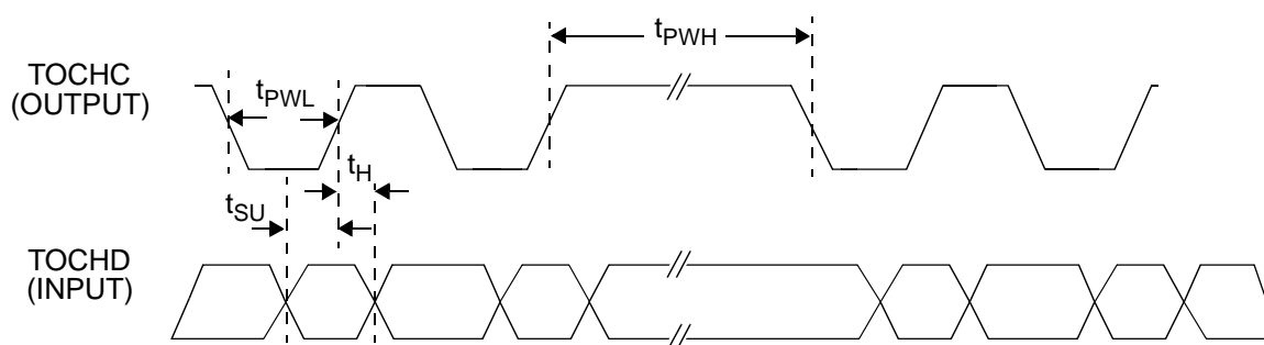
Figure 23. Transmit Overhead Communications Channel Timing
