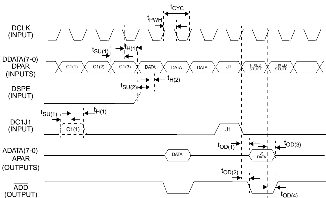
Figure 17. STS-3 Add/Drop Bus Interface Timing
