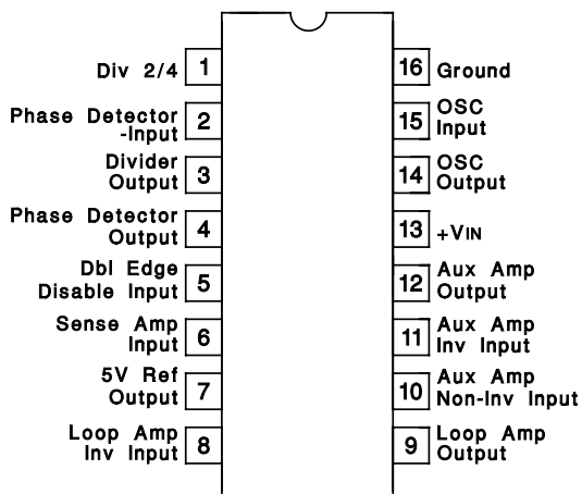
DIL-16 (Top View) J & N Packages
