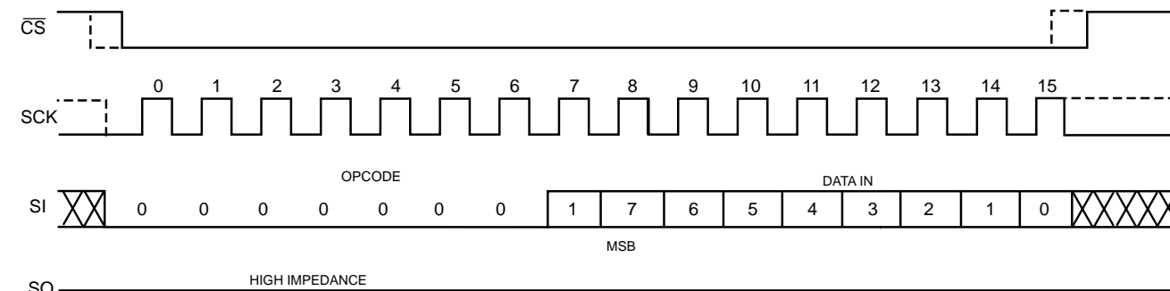
Figure 7. WRSR Timing
