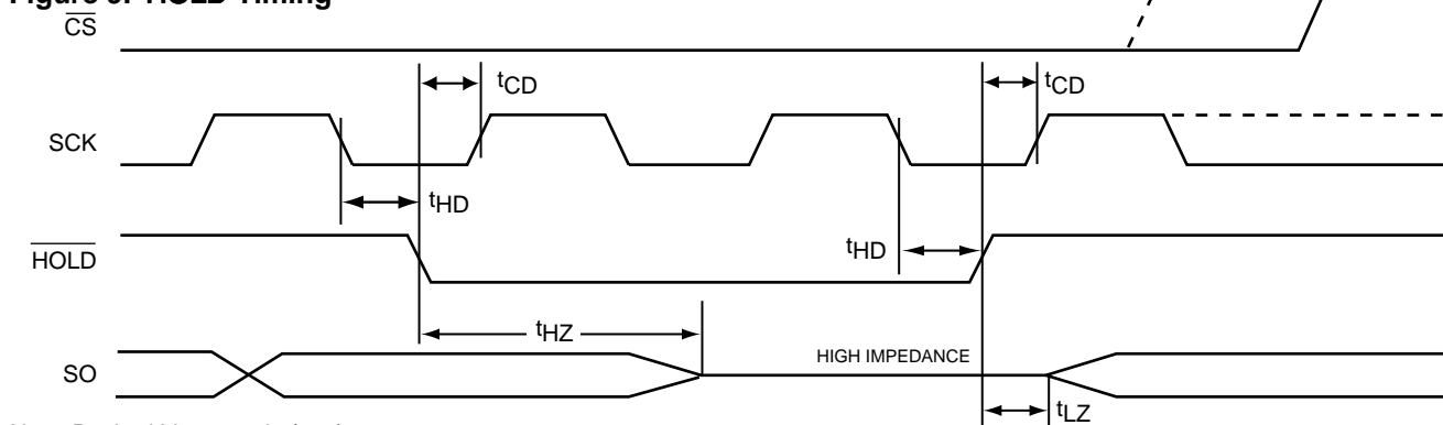
Figure 9. HOLD Timing
