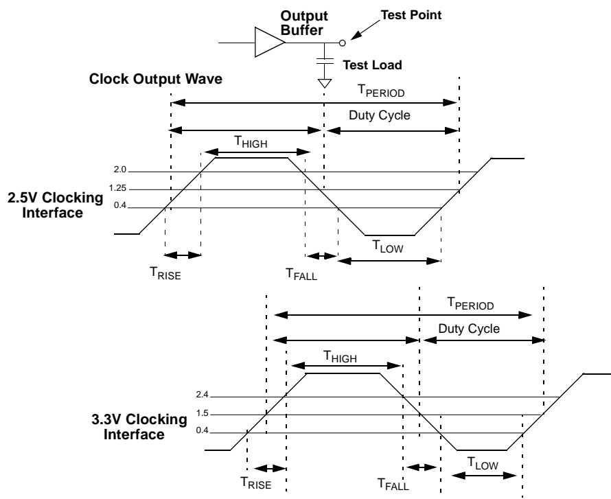
Figure 10. Output Buffer
