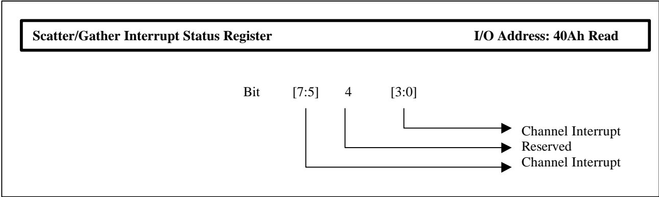
Scatter/Gather Interrupt Status Register (default = 00h)
