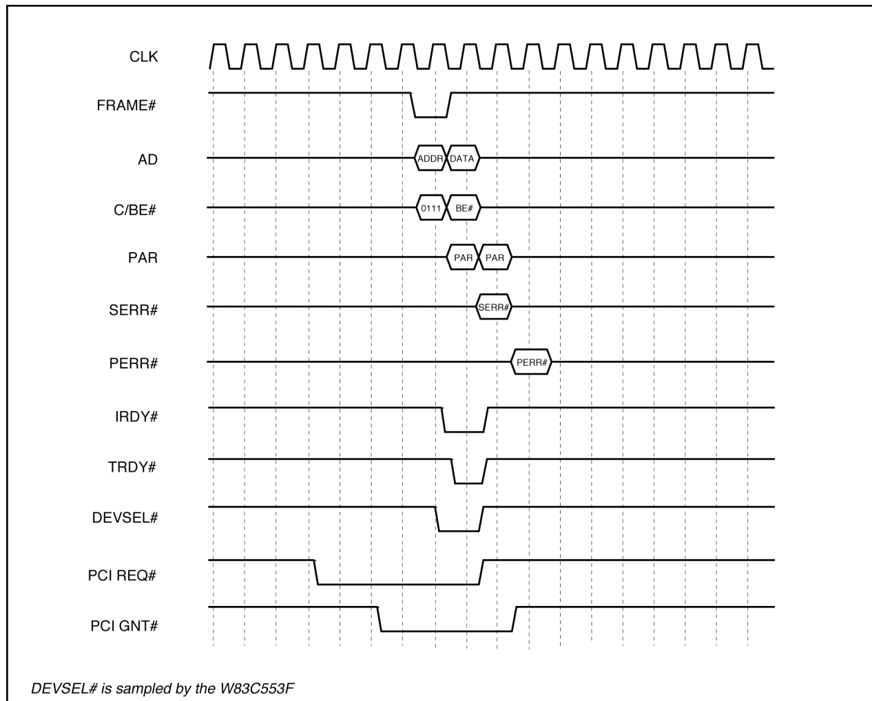
Figure 3-7. Master Memory Write
