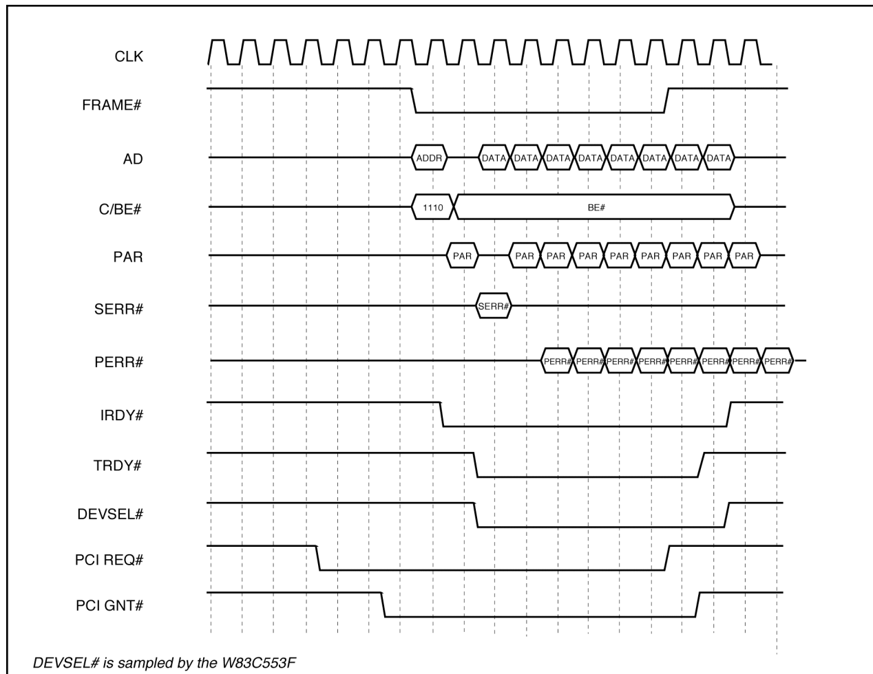
Figure 3-8. Master Memory Read Line
