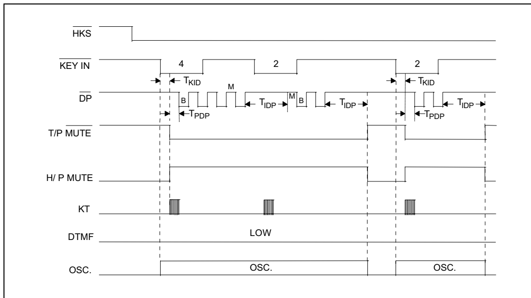
Figure 1(a) Pulse Mode Timing Diagram (Normal dialing without lock function)
