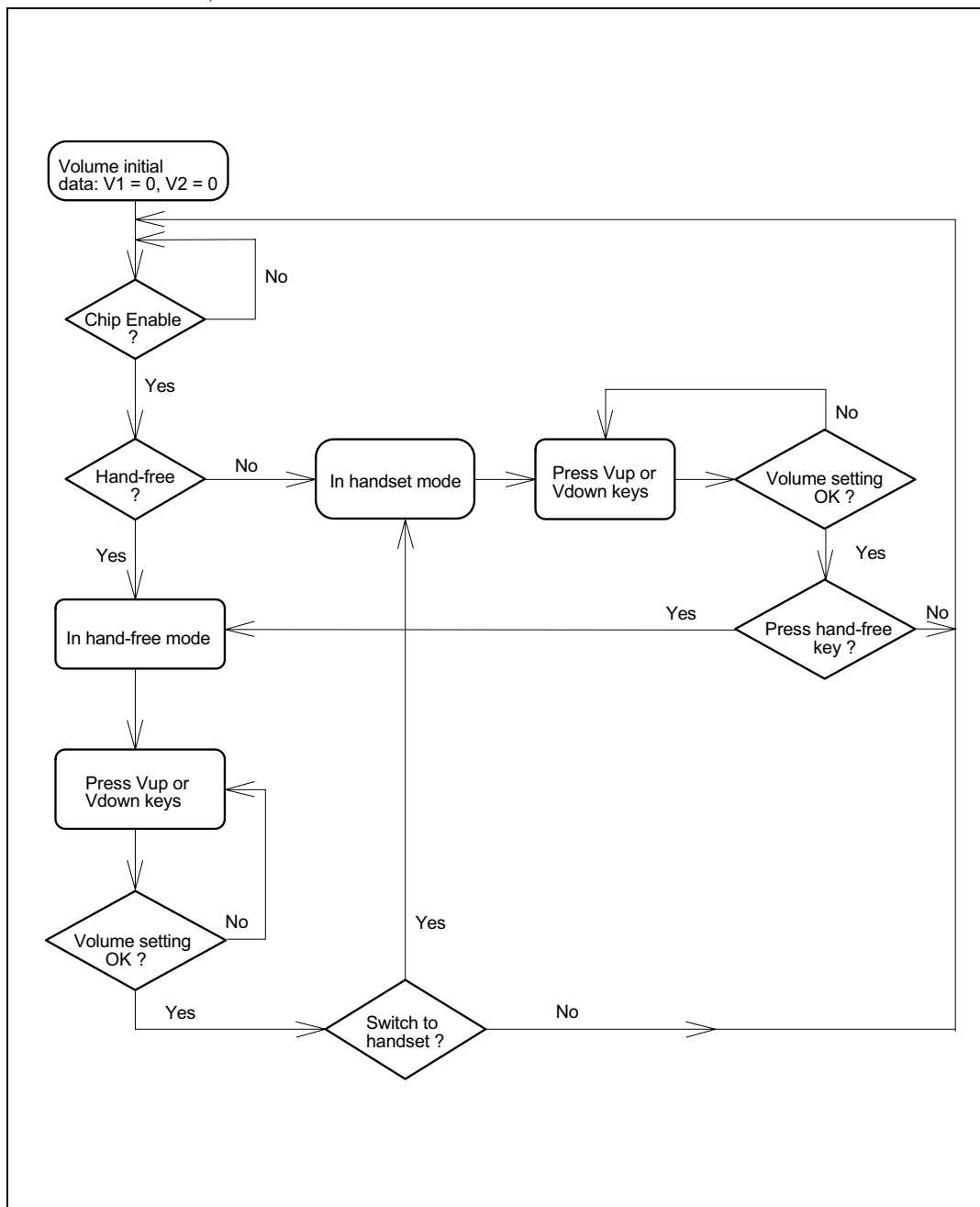
Volume Control Flow Chart, continied
