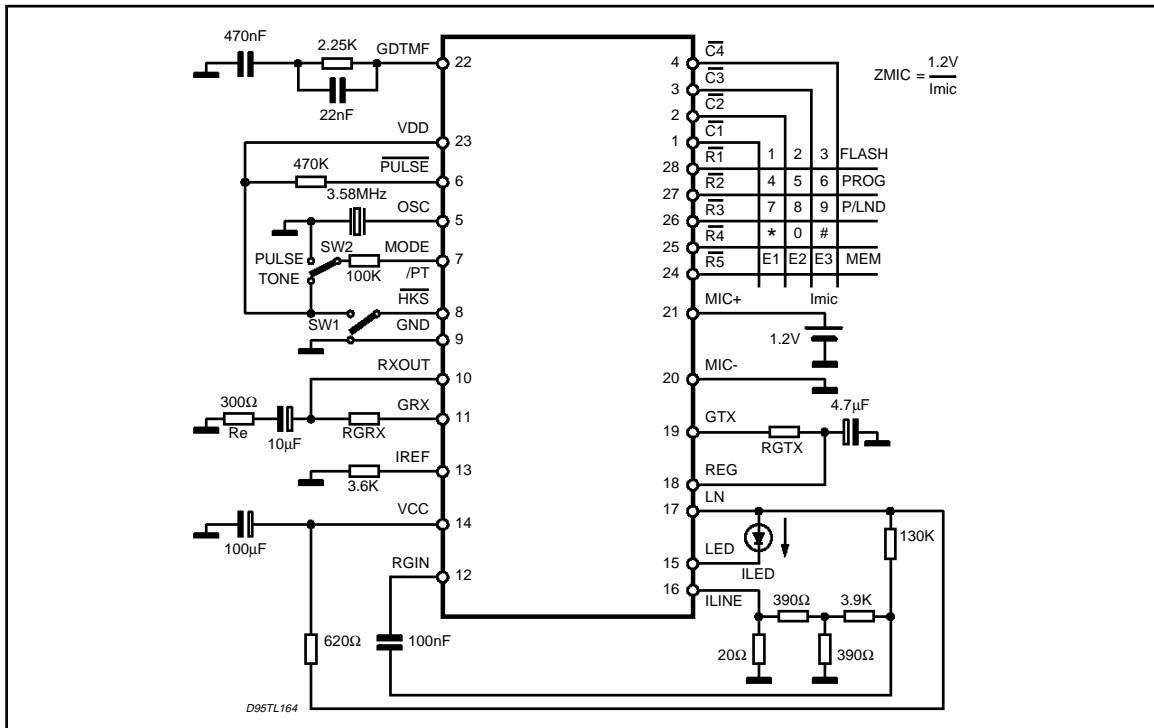
TEST CIRCUITS(continued) Figure 5.
