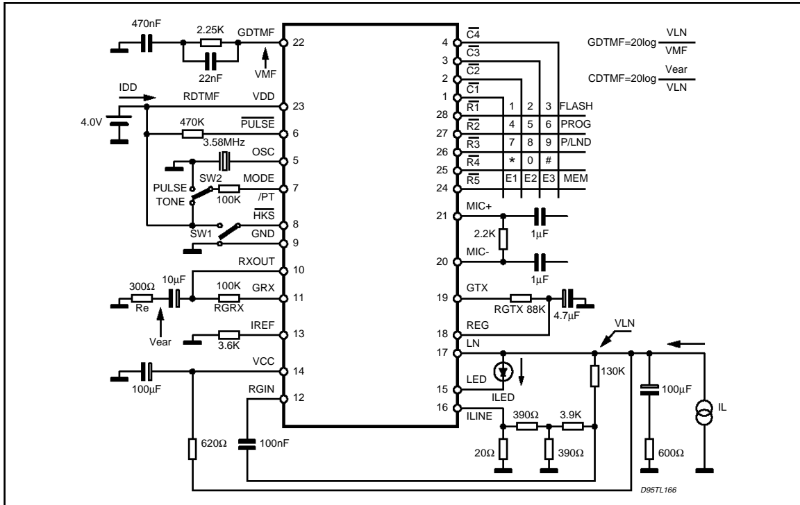
TEST CIRCUITS(continued) Figure 7.
