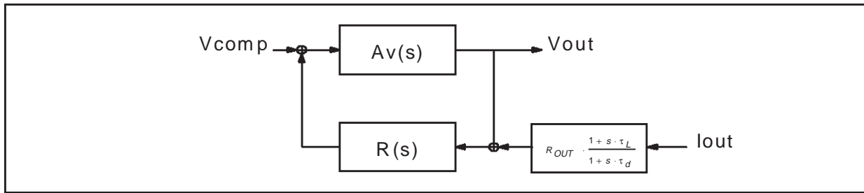
Figure 9. Voltage regulation with droop function block scheme
