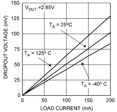
Dropout Voltage
