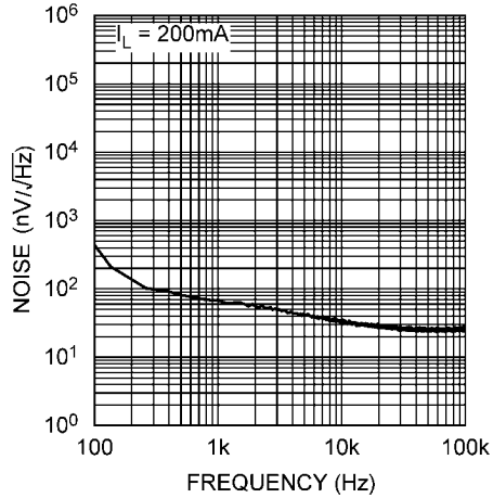
Noise Density
