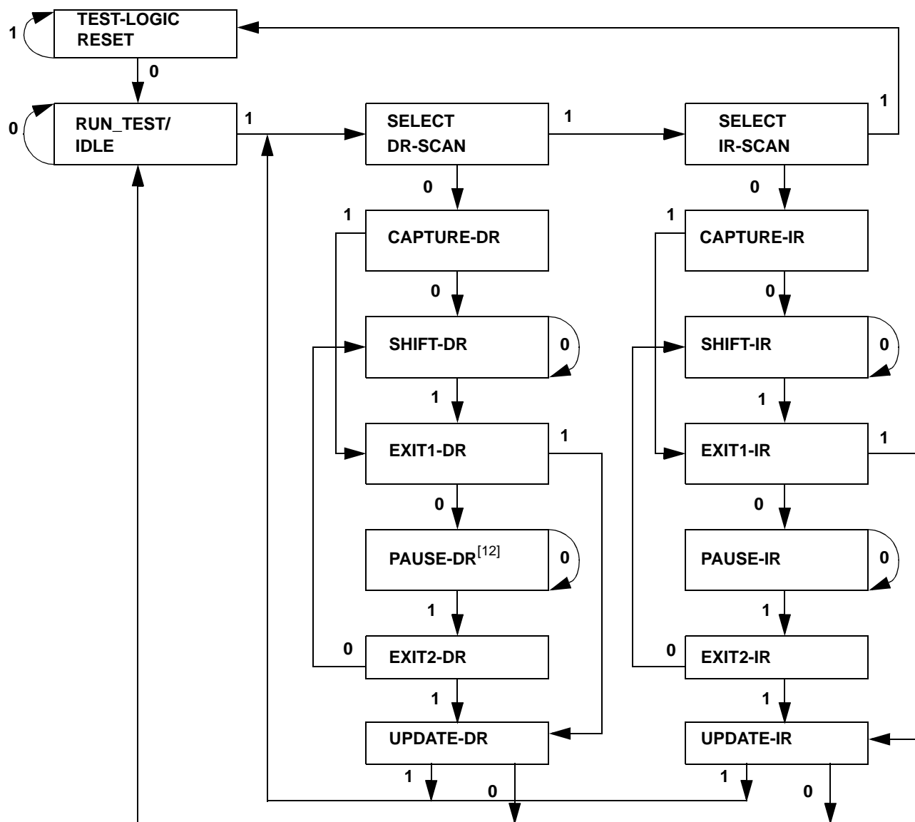
Figure 3. TAP Controller State Diagram (FSM) [14]
