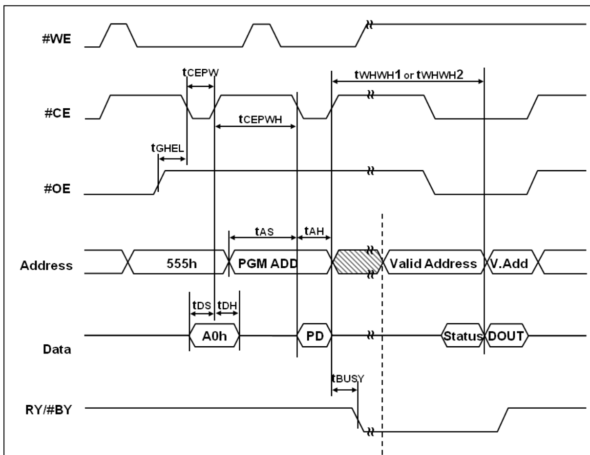
Figure 8-15 CE# Controlled Write Timing Waveform
