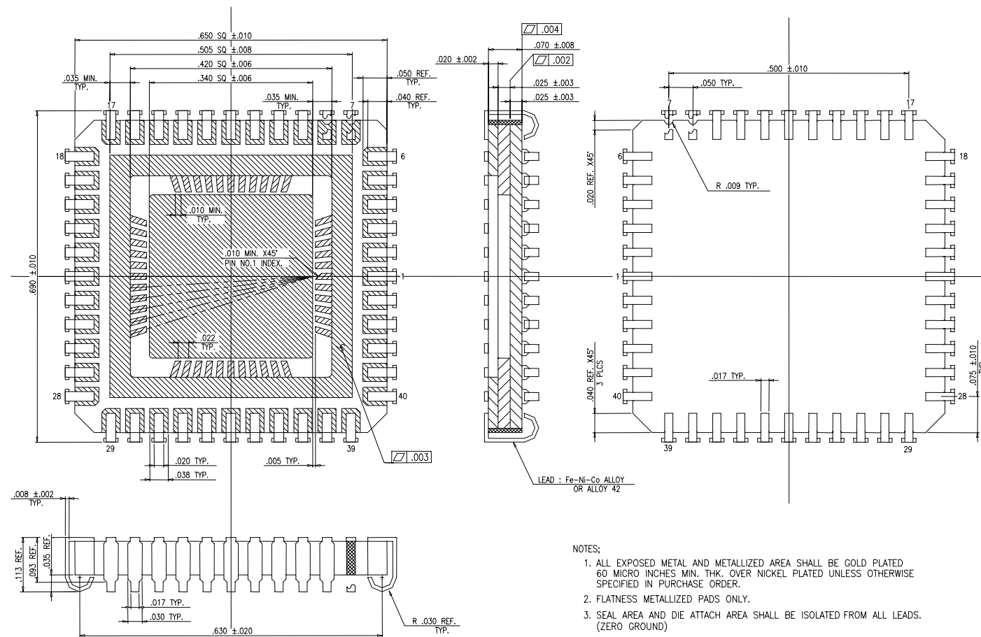
Figure 6. Package Drawing
