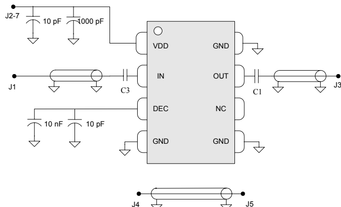
Figure 10. Evaluation Board Schematic Diagram
