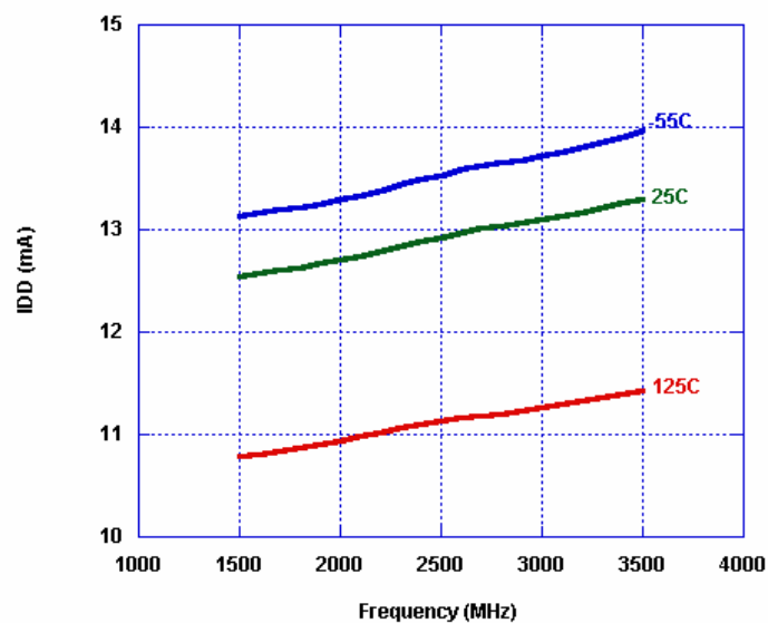
Figure 5. Device Current
