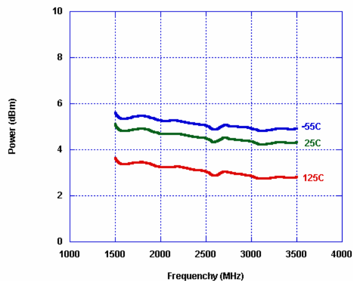
Figure 6. Output Power
