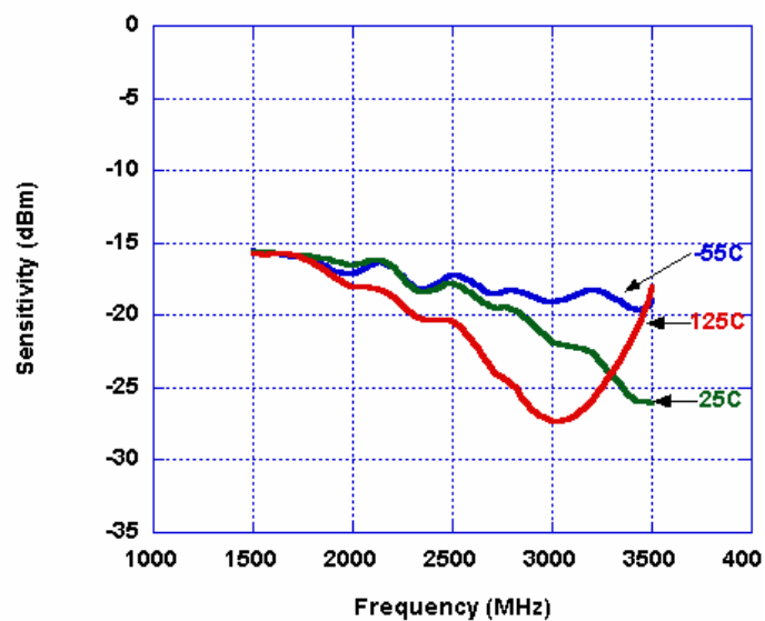
Figure 4. Input Sensitivity
