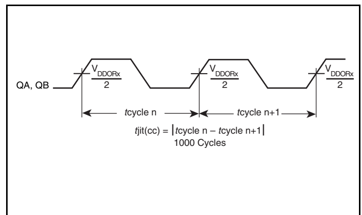
Cycle-to-Cycle Jitter
