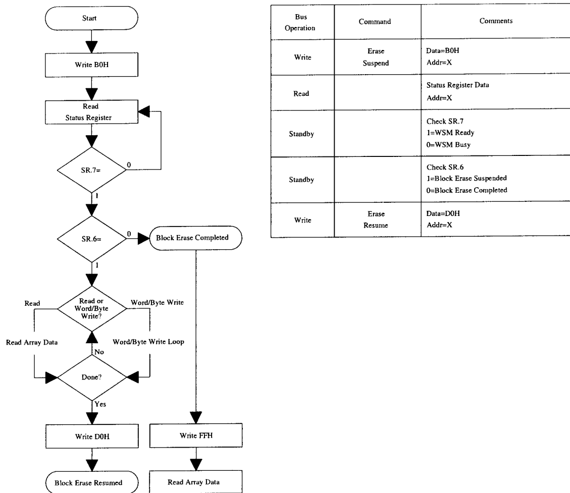
Figure 7. Block Erase Suspend/Resume Flowchart
