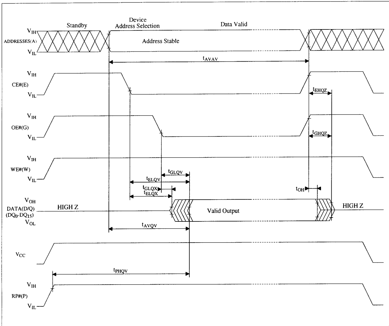
Figure 11. AC Waveform for Read Operations
