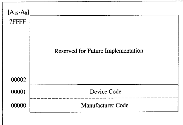
Figure 4. Device Identifier Code Memory Map
