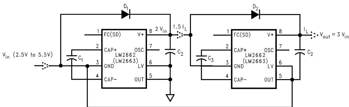
FIGURE 7. Generating +3V_{in} from +V_{in}
