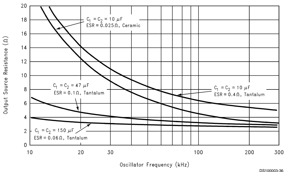
FIGURE 3. Output Source Resistance vs Oscillator Frequency
