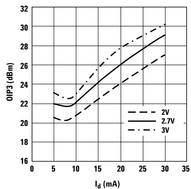
Figure 8. OIP3 vs. I_{ds} and V_{ds} at 900 MHz [1] .
