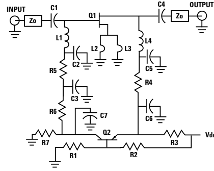
Figure 2. Typical ATF-551M4 LNA with Active Biasing.
