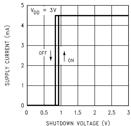
Shutdown Hysteresis Voltage V_{DD} = 3V
