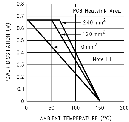
Power Derating - 8 Bump \mu SMD P_{DMAX} = 670mW for 5V, 8\Omega
