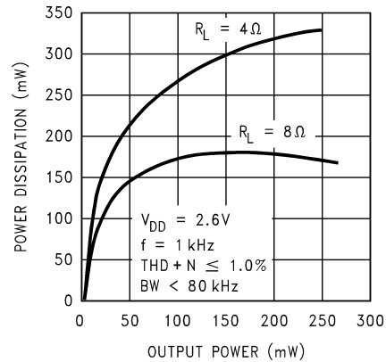
Power Dissipation vs Output Power @ V_{DD} = 2.6V
