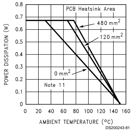
Power Derating - 9 Bump \mu SMD P_{DMAX} = 670mW for 5V, 8\Omega
