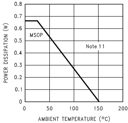
Power Derating - MSOP P_{DMAX} = 670mW for 5V, 8\Omega
