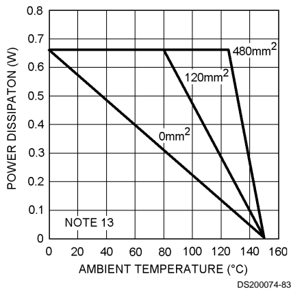
Power Derating - 10 Pin LD Pkg P_{DMAX} = 670mW , 5V, 8Ω
