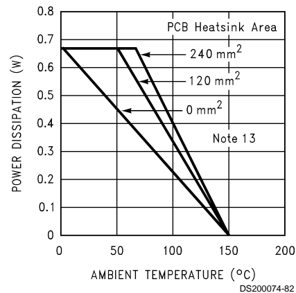
Power Derating Curves for 8 Bump microSMD ( P_{DMAX} = 670mW )
