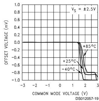
Offset Voltage vs V_{CM}
