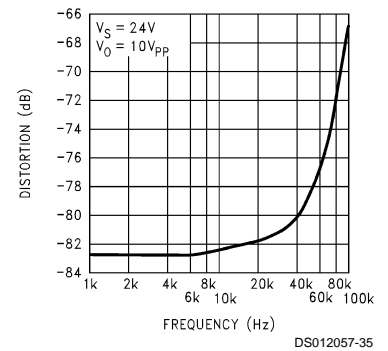
Distortion + Noise vs Frequency
