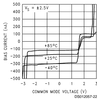
Bias Current vs V_{CM}
