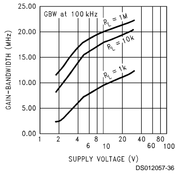
GBW vs Supply
