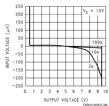
Open-Loop Transfer Function
