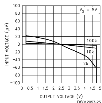
Open-Loop Transfer Function
