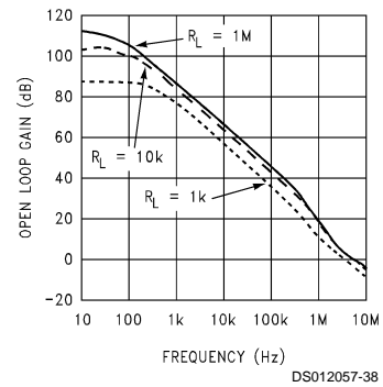
Open Loop Gain vs Load, 5V Supply
