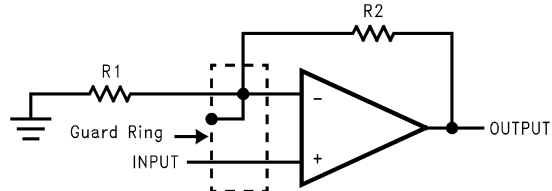
(b) Non-Inverting Amplifier
