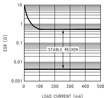
10133938 Stable Region For output Capacitor ESR
