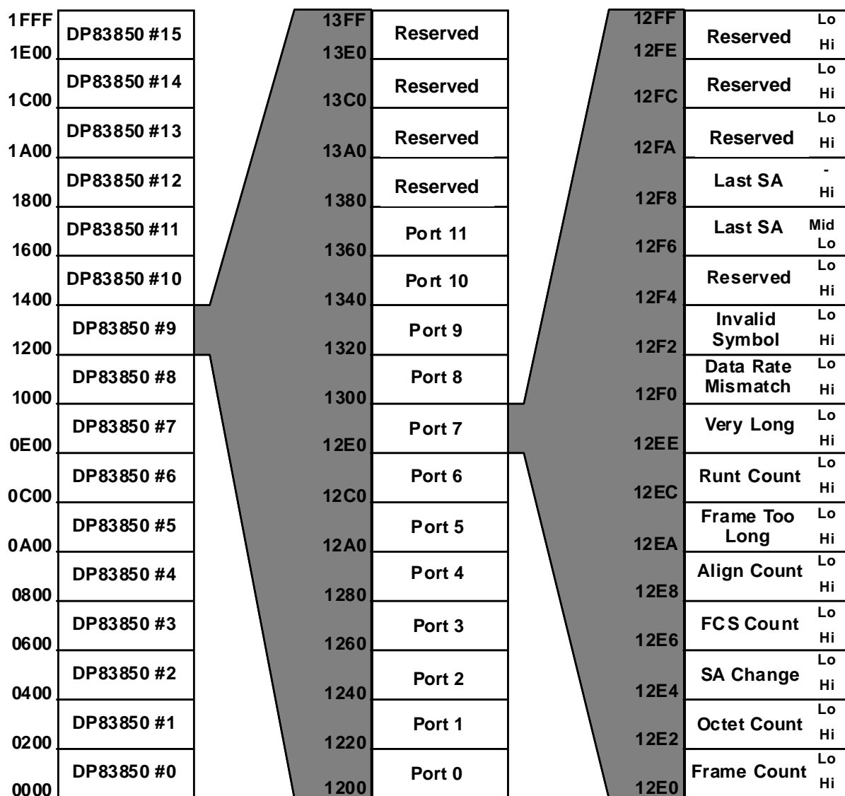
Figure 1. Memory Map for the DP83856 Statistics SRAM
