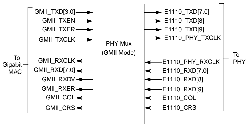
Figure 2.3 PHY Multiplexer Signal Mapping in GMII Mode
