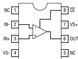
EL5192ACS (8-Pin SO)
