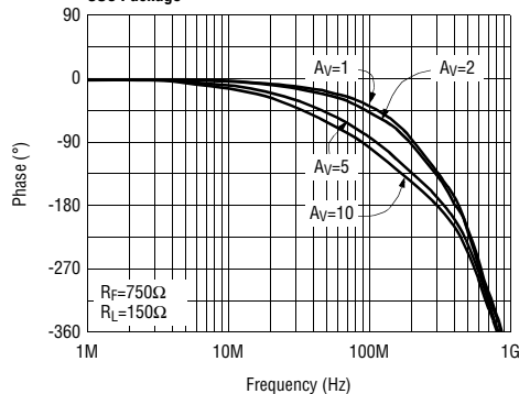
Non-inverting Frequency Response (Phase) S08 Package
