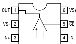
EL5192ACW (6-Pin SOT-23)
