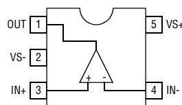
EL5192CW (5-Pin SOT-23)
