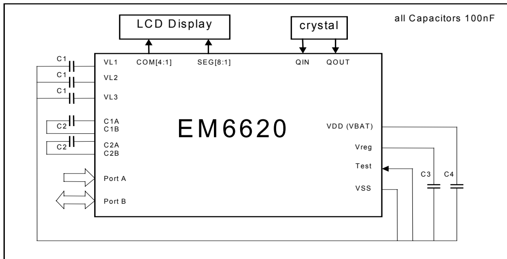
Figure 3. Typical configuration
