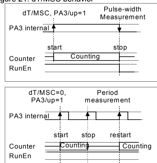
Figure 21. dT/MSC behavior
