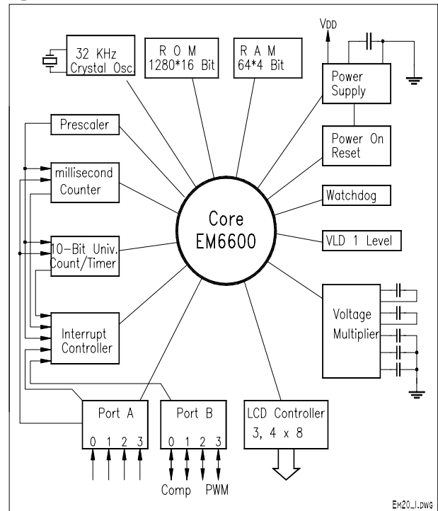
Figure 1. Architecture
