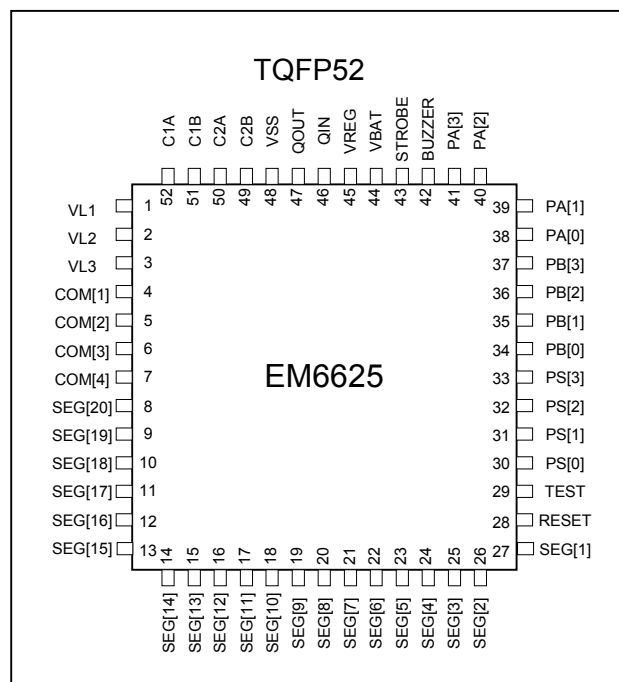
Figure 2. Pin Configuration, TQFP52
