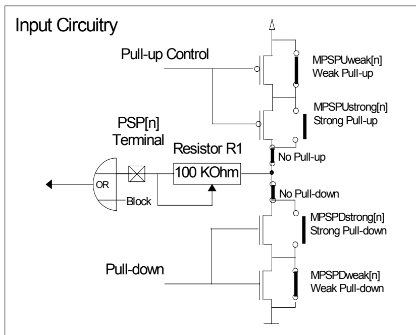
Figure 40. Port SP Pull Options
