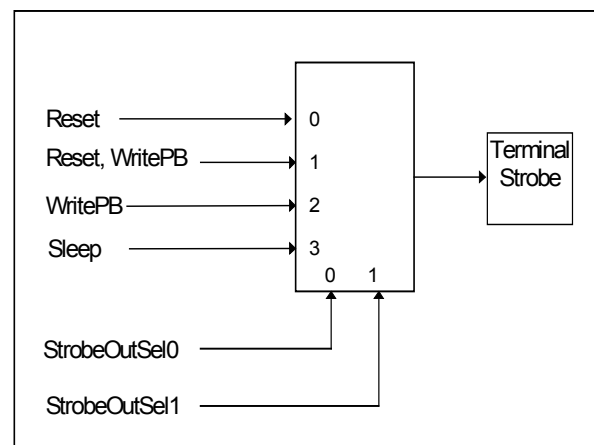
Figure 32 . Strobe Output
