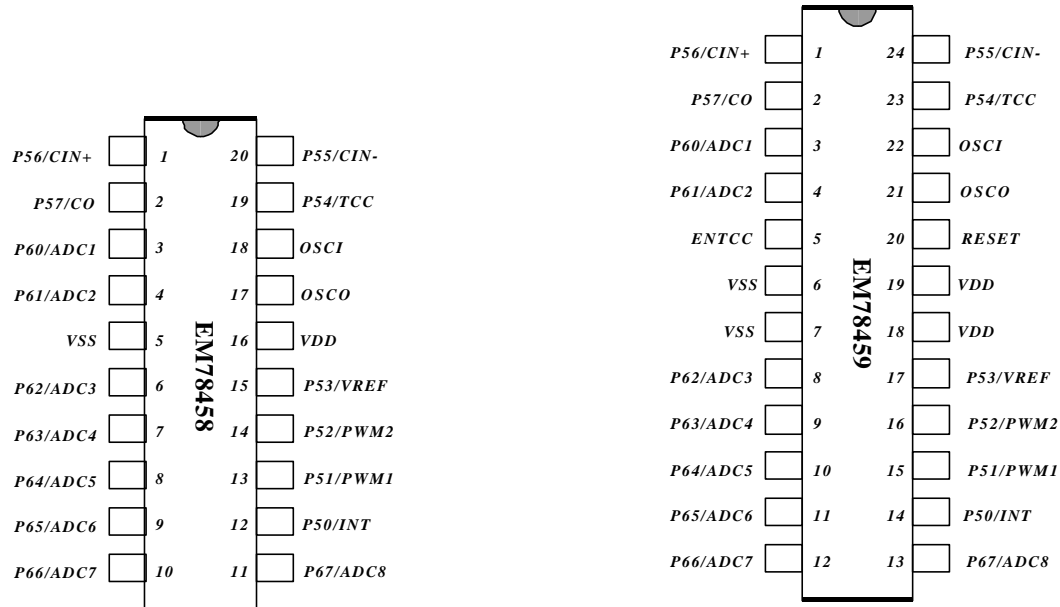
Fig. 1 Pin Assignment
