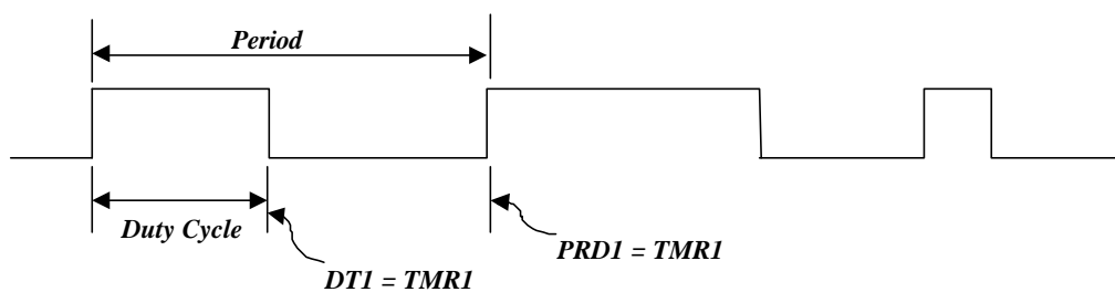
Fig. 14 The Output Timing of the PWM
