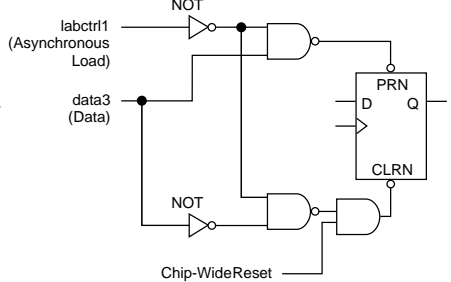
Asynchronous Load without Clear or Preset
