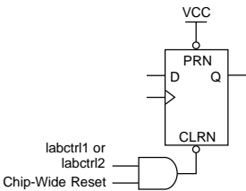
Asynchronous Clear
