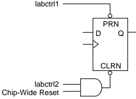
Asynchronous Preset & Clear
