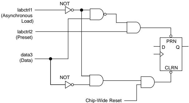
Asynchronous Load with Preset
