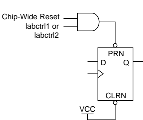
Asynchronous Preset
