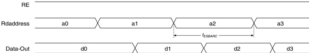
Figure 34. ESB Asynchronous Timing Waveforms
