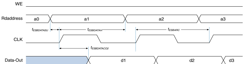
Figure 35. ESB Synchronous Timing Waveforms
