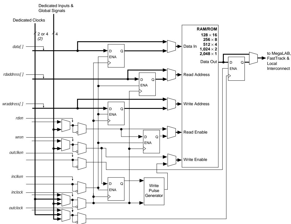
Figure 21. ESB in Input/Output Clock Mode Notes (1), (2)
