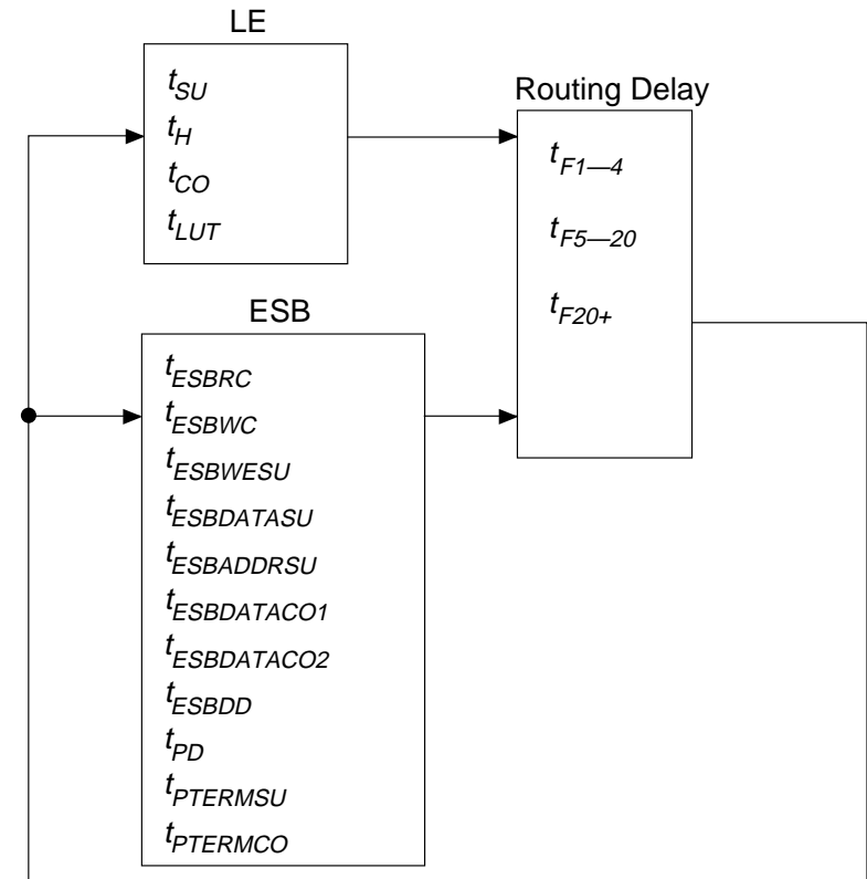
Figure 36. APEX 20K f_{MAX} Timing Model
