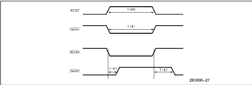
Figure 11-17. \overline{\text{SMOUT}} Timing
