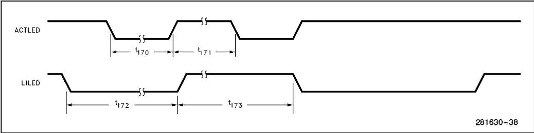
Figure 11-27. LED Timings
