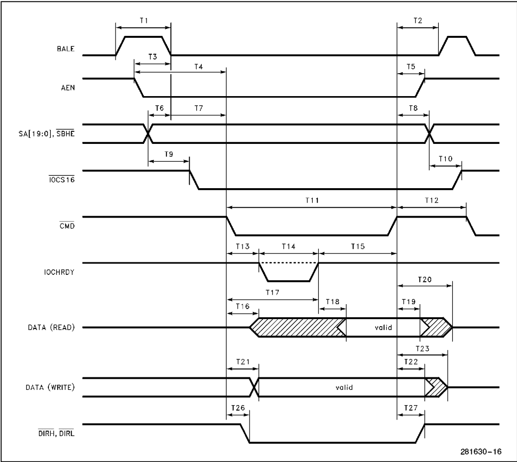
Figure 11-6. ISA-Compatible Cycle
