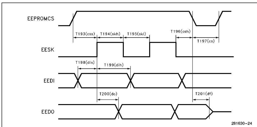
Figure 11-14. EEPROM Timings
