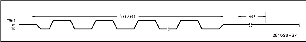
Figure 11-26. Jabber Timings
