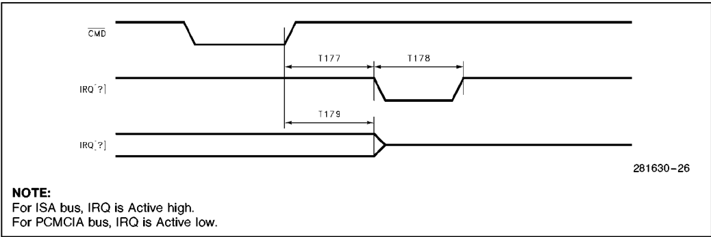
Figure 11-16. Interrupt Timing
