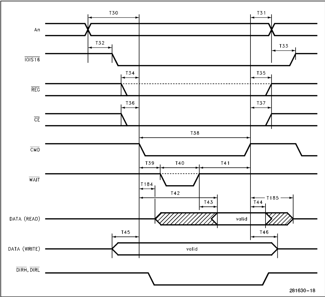
Figure 11-8. PCMCIA Cycle
