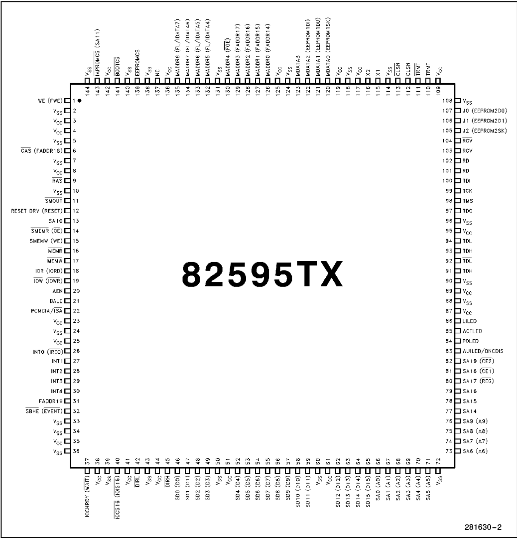
Figure 2. 82595TX Pinout
