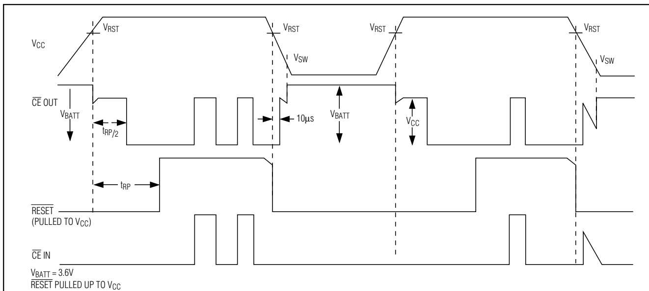
Figure 8. Chip-Enable Timing
