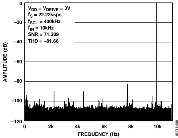
Figure 4. Typical FFT
