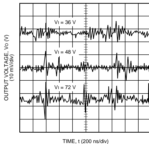
Figure 4. Typical FW300C1 Output Ripple Voltage at Room Temperature and 20 A Output
