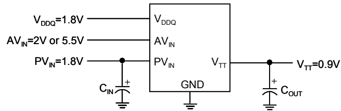
Figure 5. Recommended DDR-II Termination
