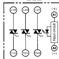
G3PB-□□□B-3-VD
