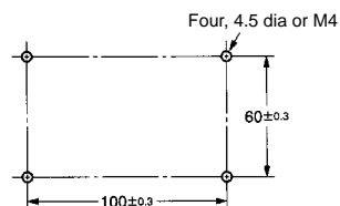
Mounting Holes
