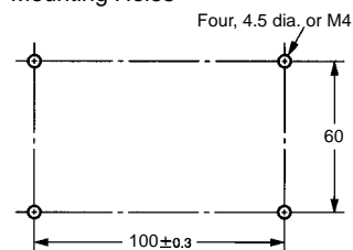
Mounting Holes
