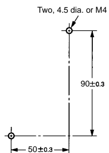
Mounting Holes
