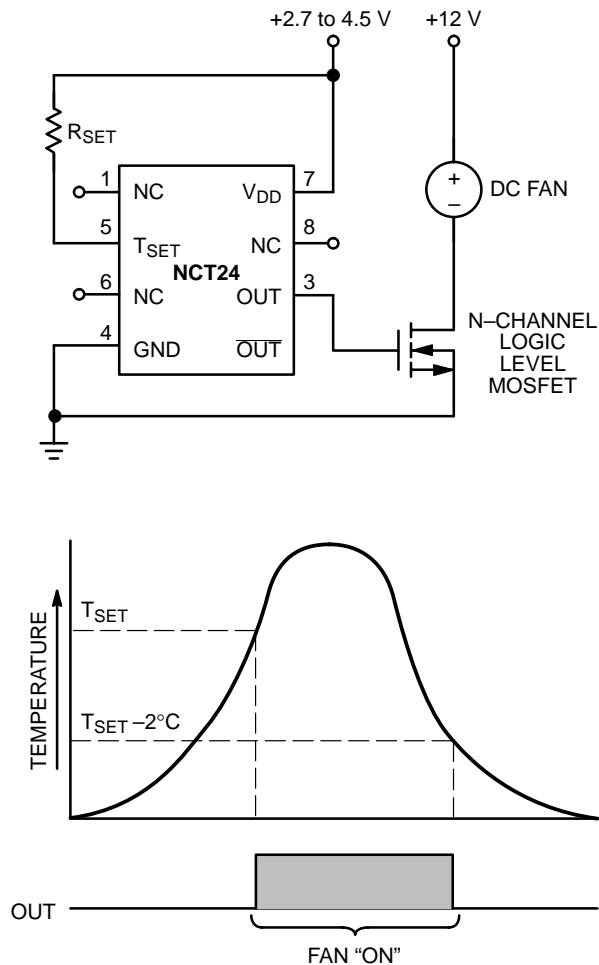
Figure 5. NCT24 As a Fan Controller for Notebook PCs
