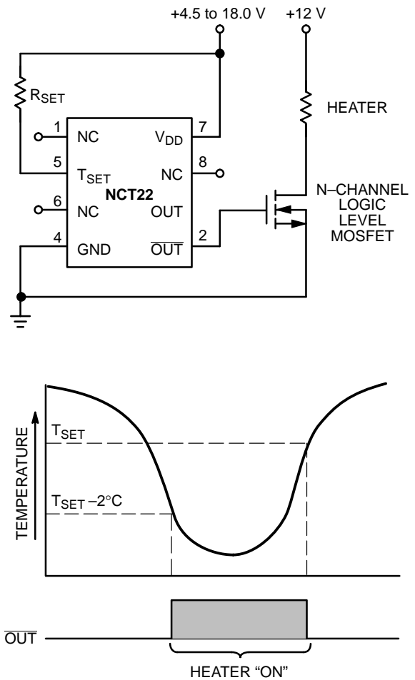
Figure 6. NCT22 As a Heater Thermostat
