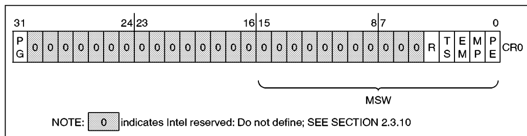
Figure 2-5. Control Register 0
