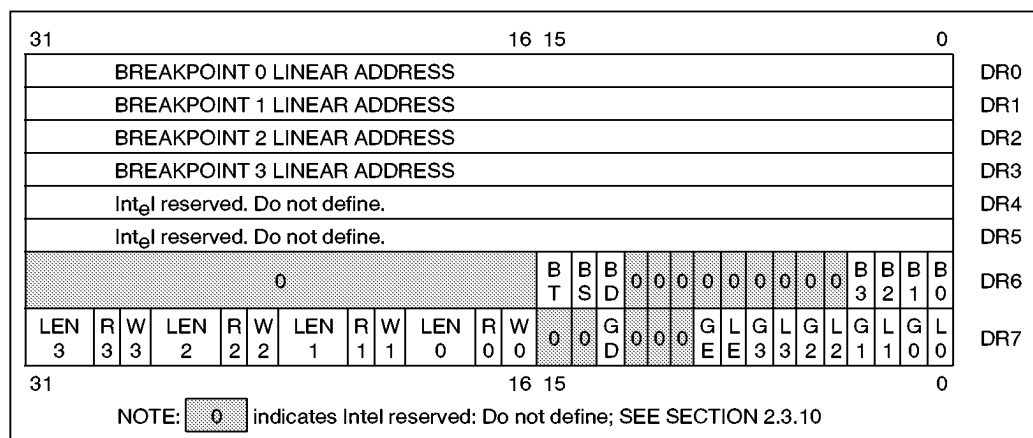
Figure 2-13. Debug Registers
