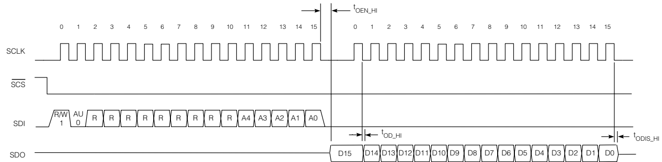
Fig. 8 Read Cycle
