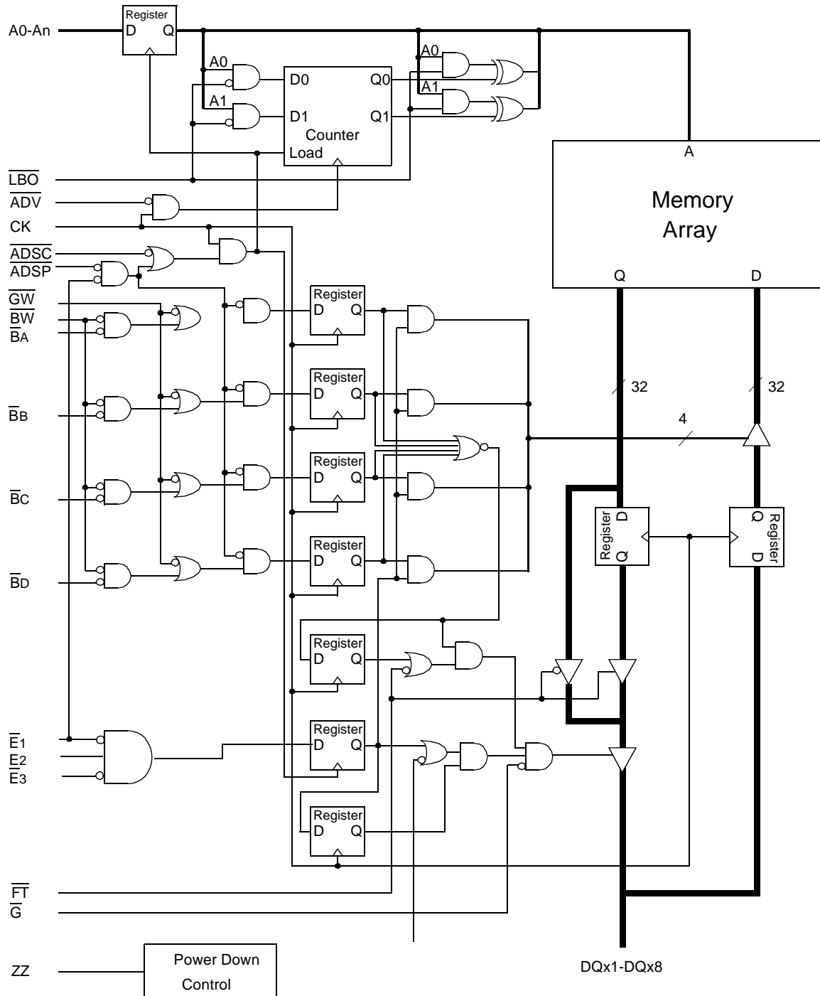
GS820E32A Block Diagram
