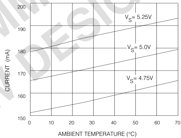
Fig. 15 Supply Current
