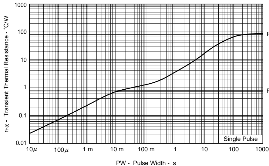
Figure5. TRANSIENT THERMAL RESISTANCE vs. PULSE WIDTH
