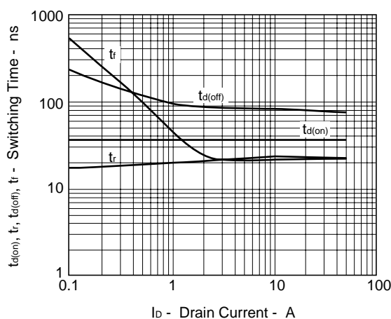
Figure15. SWITCHING CHARACTERISTICS
