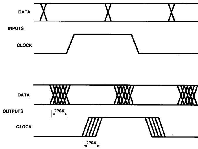
Figure 11. Parallel Data Transmission Example.
