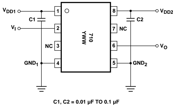
Figure 12. Recommended Printed Circuit Board Layout.
