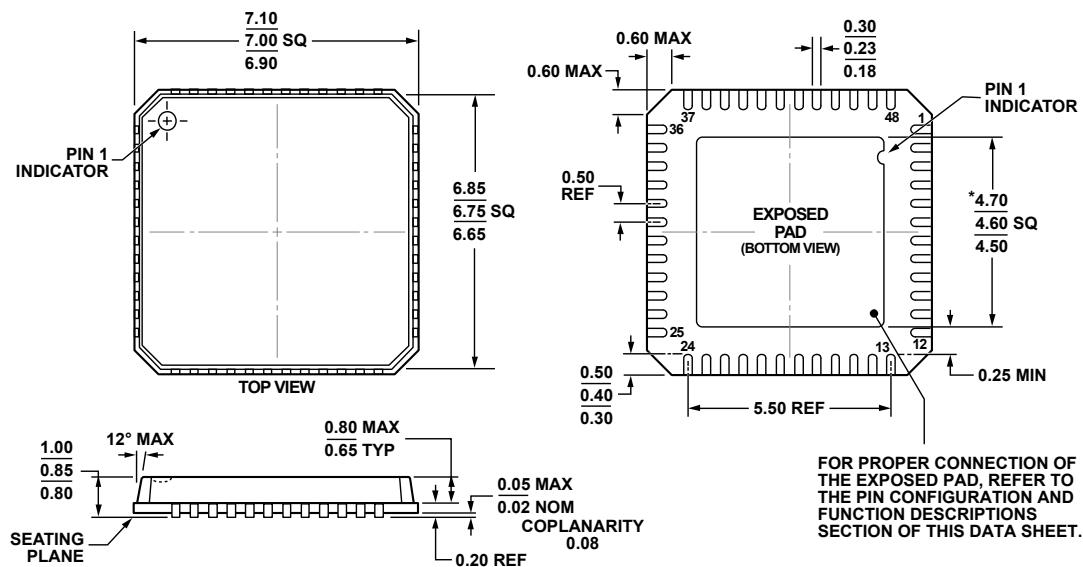
Figure 26. 48-Lead Lead Frame Chip Scale Package [LFCSP_VQ] 7 mm × 7 mm Body, Very Thin Quad (CP-48-12)
