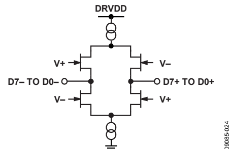
Figure 18. LVDS Output Driver
