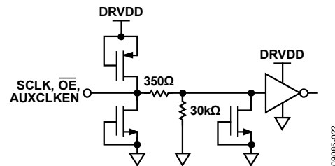
Figure 16. SCLK, \overline{OE}
