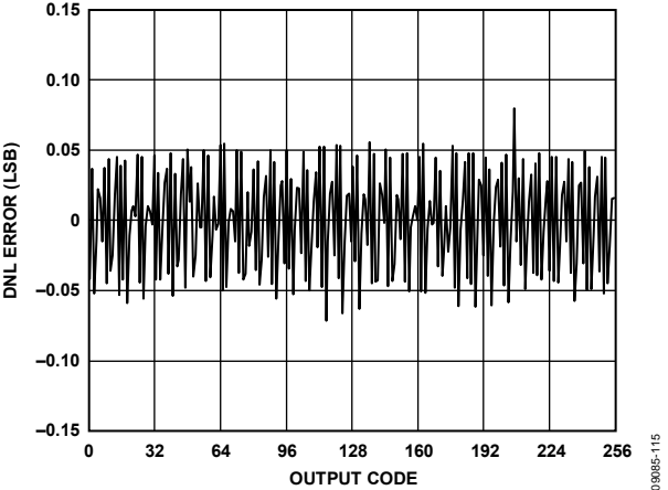
Figure 11. DNL Error with f_{IN} = 4.3 MHz
