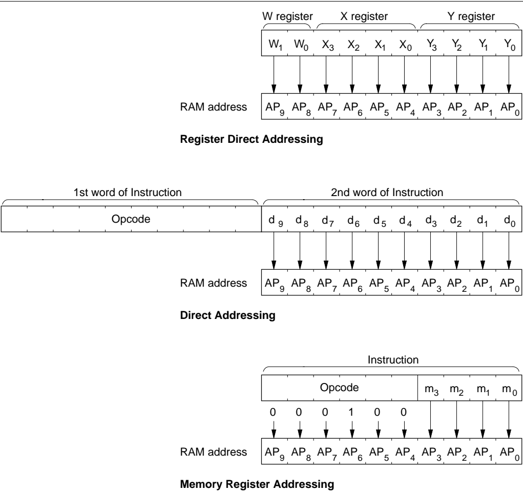
Figure 100 RAM Addressing Modes
