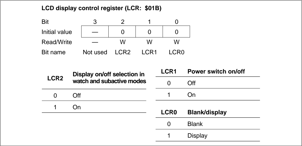
Figure 89 LCD Control Register (LCR)
