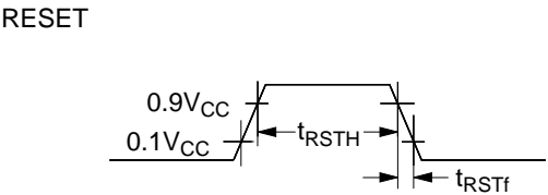
Figure 106 Reset Timing
