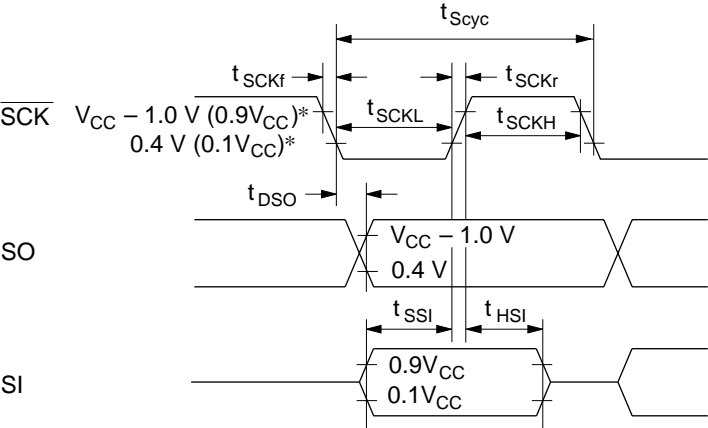
Figure 107 \overline{\text{STOPC}} Timing
